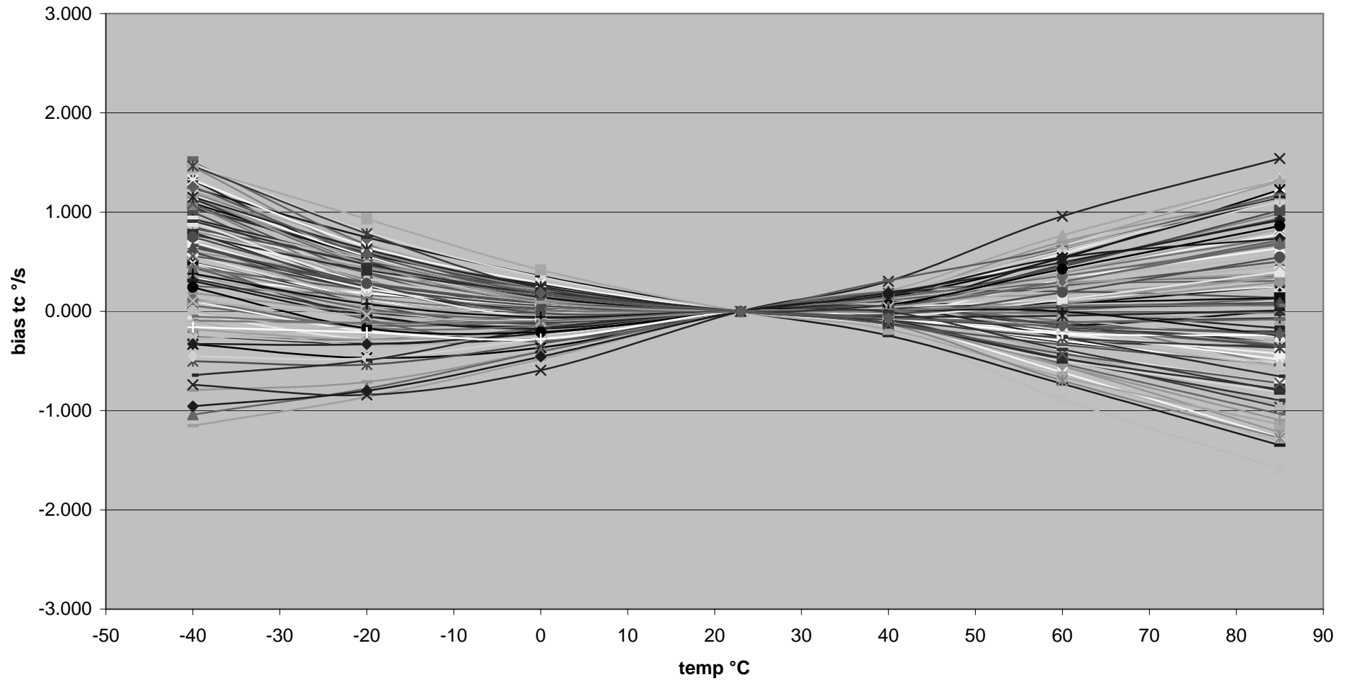
CRS03-02 bias tc - normalised at 23°C (100 units randomly selected from Feb 04 production) (specification limit \pm 3^\circ/\text{s} )
