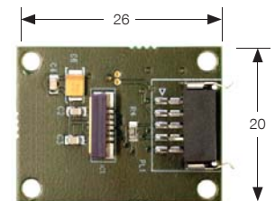
Orion™ Evaluation Board - CMS390 (P/N CMS390-02-0302)
